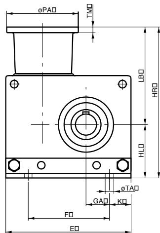
Mounting position VV, VH, VD
