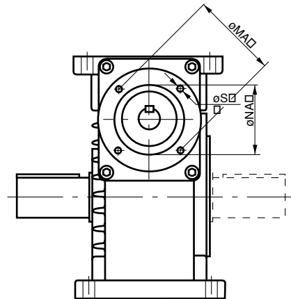
Mounting position OV
