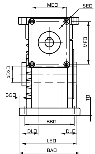
Mounting position O-hollow shaft
