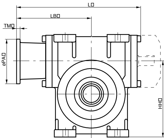
Mounting position OH, OV, OD
